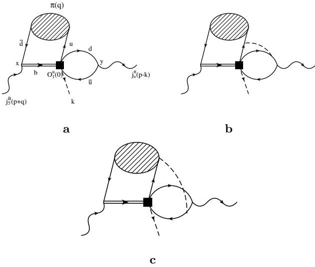
Fig. 1. Contributions in the emission topology: a factorizable contribution from the \mathcal{O}_1^u operator; b an example of the \mathcal{O}(\alpha_s) correction; c an example of the nonfactorizable diagram from the \tilde{\mathcal{O}}_1^u operator
